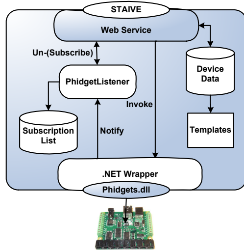
Figure 6. Phidgets FDX
